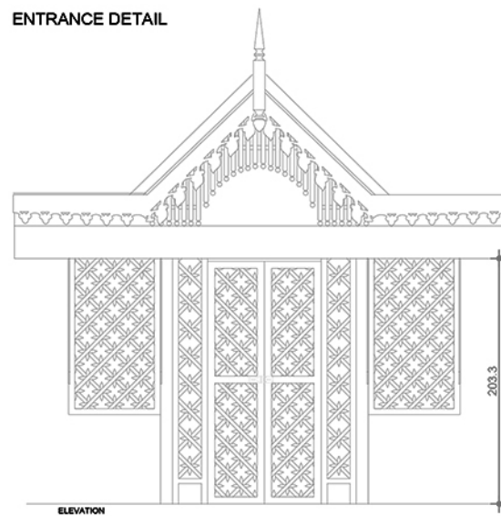
ENTRANCE DETAIL
