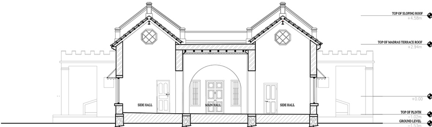
SECTION 2-2
